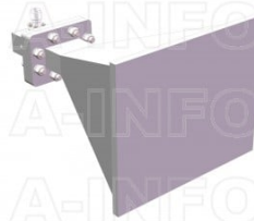
LB-137-15-C-TFSPO Standard Gain Horn Antenna 5.85-8.2GHz 15dB Gain TNC Female
