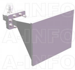
LB-137-15-C-7SPO Standard Gain Horn Antenna 5.85-8.2GHz 15dB Gain 7mm
