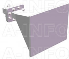
LB-137-15-C-SFSPO Standard Gain Horn Antenna 5.85-8.2GHz 15dB Gain SMA Female
